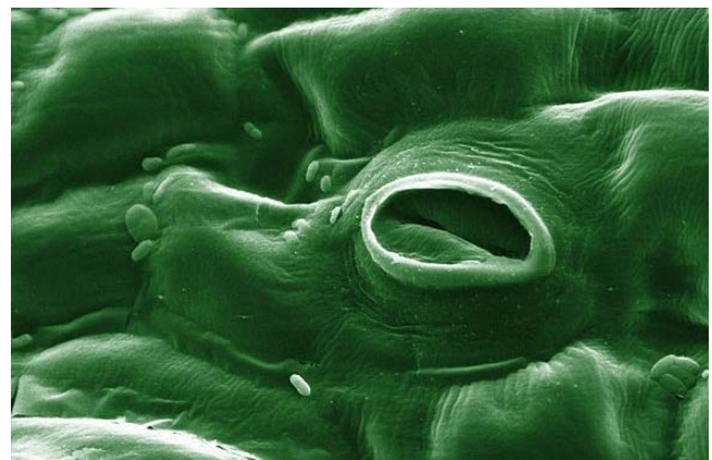
Figure 3. Electron microscope image of a stoma on the leaf of a tomato plant.
