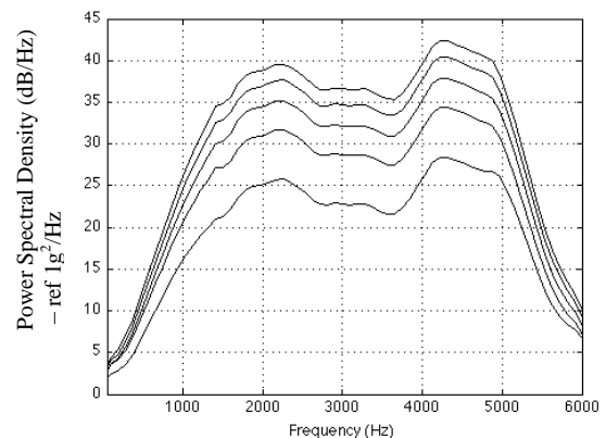
Figure 4. Response of the wooden panel at location L4 for five different amplitudes. For each amplitude level, the plot corresponds to the mean value of 20 measurements.
