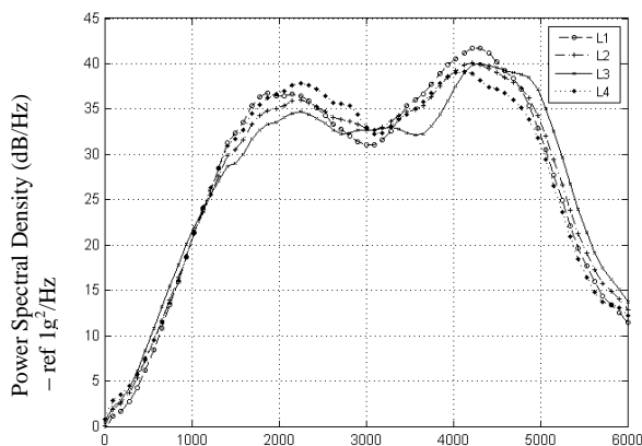
Figure 5. Response of the haptic display at locations L1, L2, L3, and L4 at one amplitude level.
