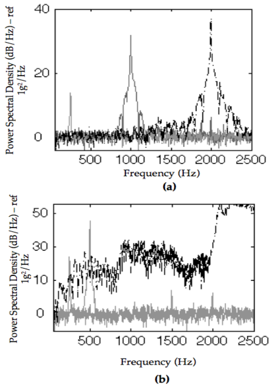
Figure 8. Image (a), shows a valid trial. In this case, the Power Spectral Density (PSD) of the ‘detected’ stimuli (sine tone) at 2000 Hz (dashed black line with a peak at 2000 Hz) is more than 15dB below the lowest threshold of detectability (solid grey lines): sine tone at 1000 Hz and sine tone at 250 Hz for the same subject. Image (b) shows an invalid trial due to the presence of subharmonics. In this case, the PSD of the ‘detected’ stimuli (FM tone) at 2000 Hz (dashed black line) produces low frequency components within 10dB of the lowest detectable thresholds (grey lines): sine tone at 500 Hz and sine tone at 250 Hz for the same subject.
